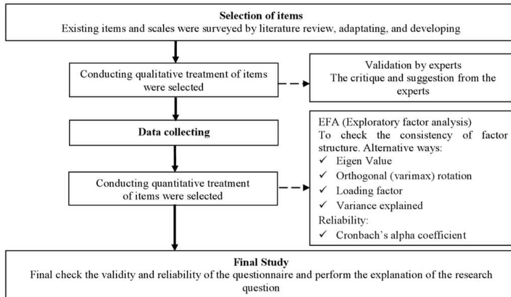
Figure 1. The process of survey study
